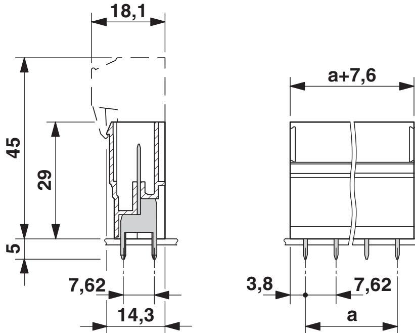
Dimensional drawing
