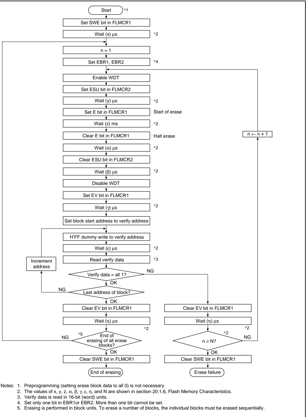
Figure 17.22 Erase/Erase-Verify Flowchart (Single-Block Erase)
