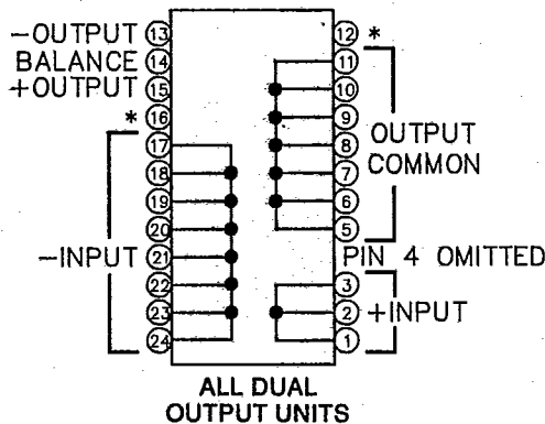
TOP VIEW VB
