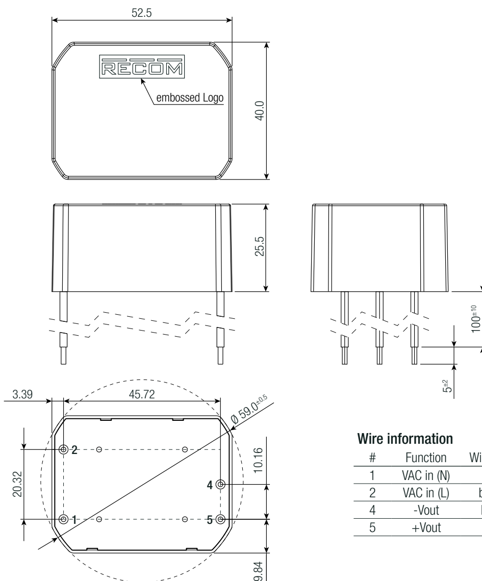
Dimension Drawing Wired version "/W" SINGLE Output (mm)
