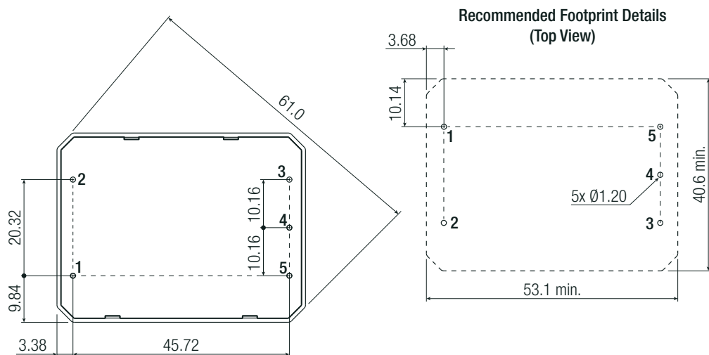
Pinning information [P12]
