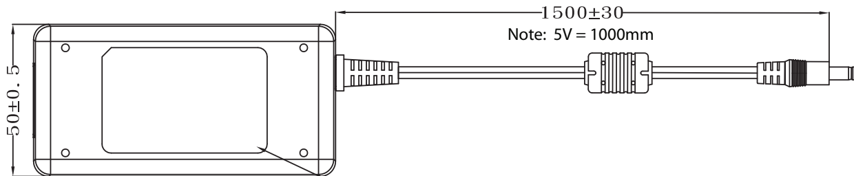
BOTTOM VIEW
