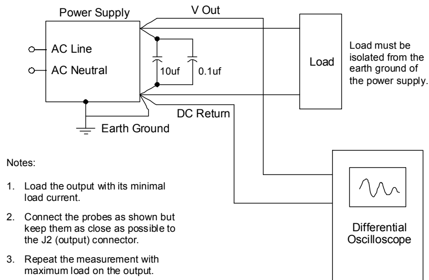
Figure 3-2 Ripple Noise Measurement Setup
