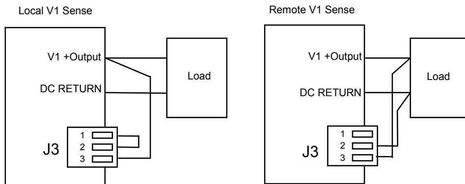
Figure 3-5 Local and Remote Sensing Wiring: Single Output Models (-12 through -48)
