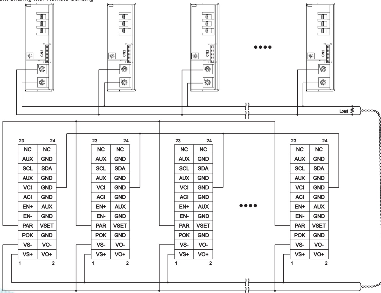
3. Current Sharing with Remote Sensing
