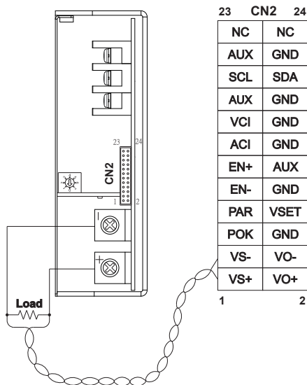
3. Current Sharing with Remote Sensing
