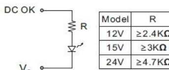
(b) LED
