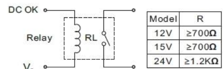
(c) Relay
