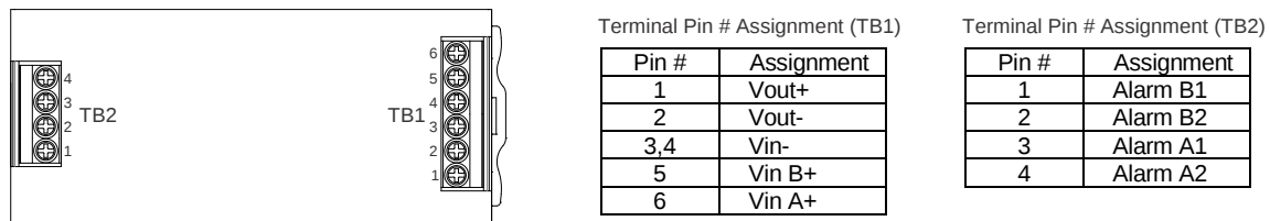
Figure 3-8 DLRDM20 Terminal Block Pin Assignments
