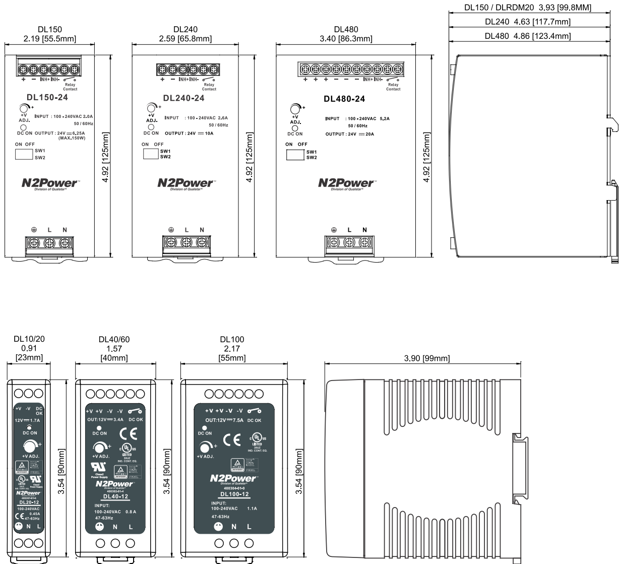
Figure 4-2 DL Dimensions
