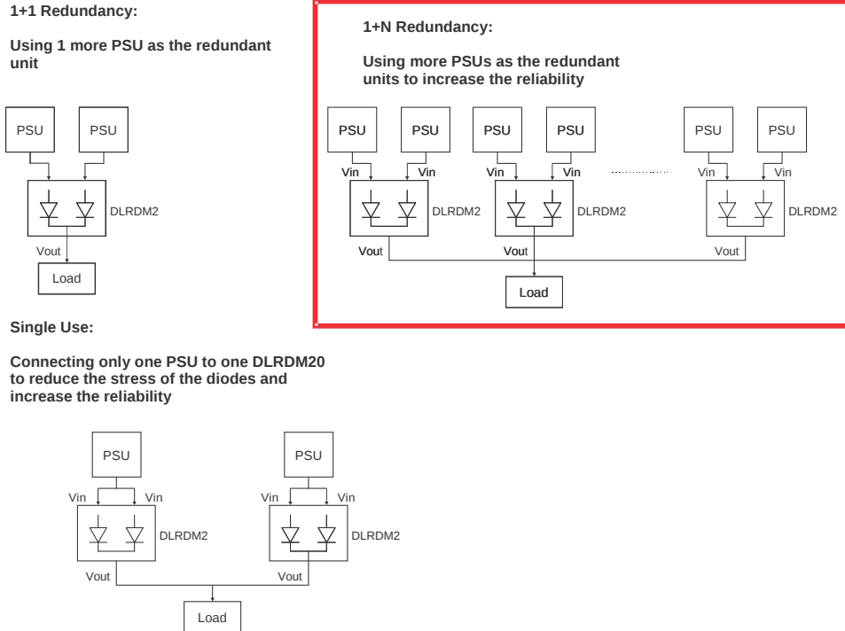
Figure 3-7 DLRDM20 Typical Applications
