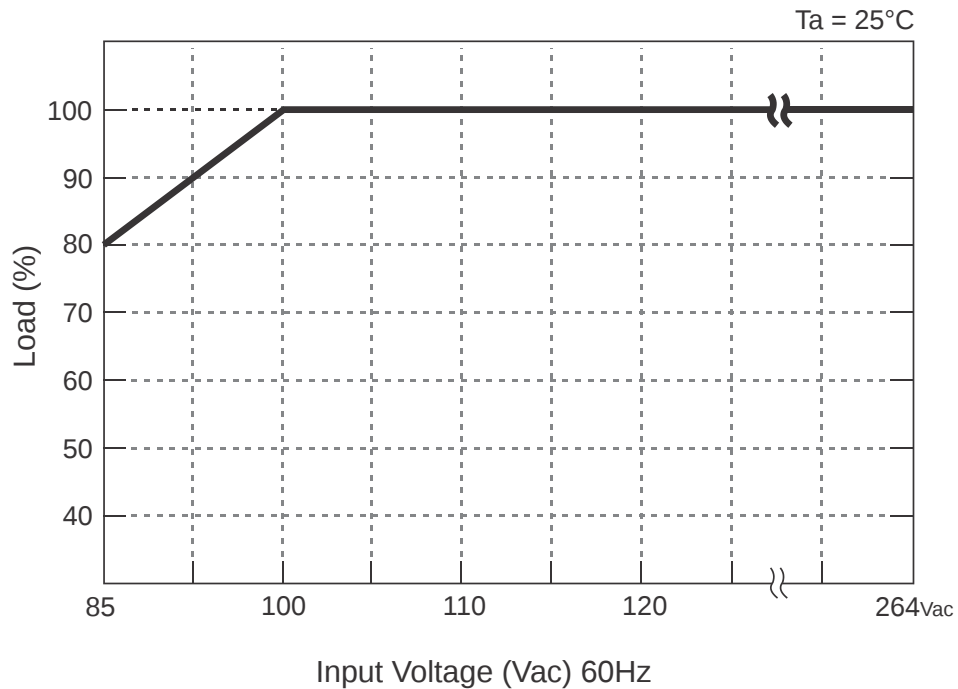
Figure 3-2 Load vs. Input Voltage: DL10 thru DL100 Series
