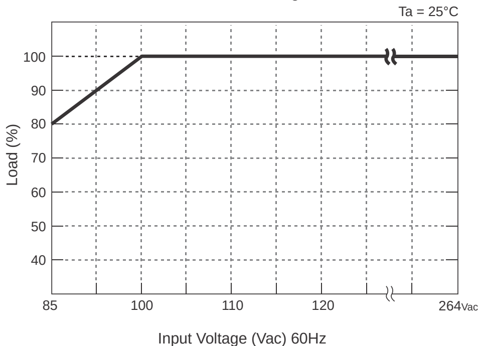
Load vs. I/P Voltage
