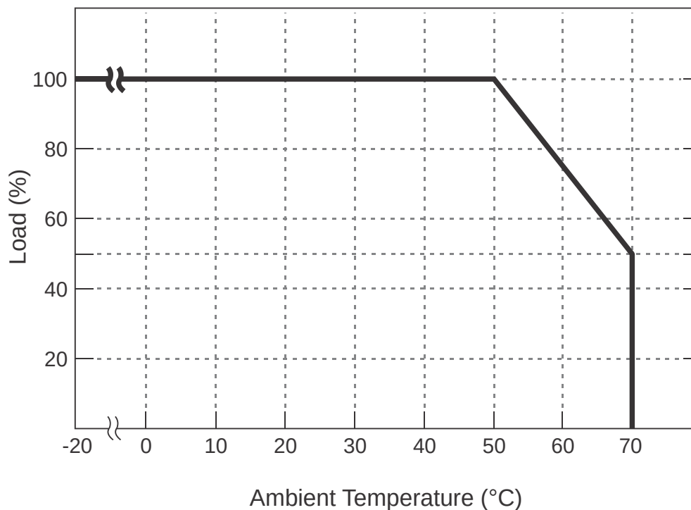
Figure 3-1 Derating Curve: Models DL10 thru DL100 Series
