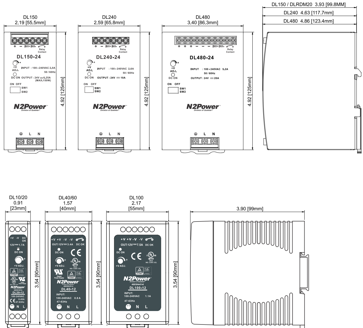
Figure 4-2 DL Dimensions
