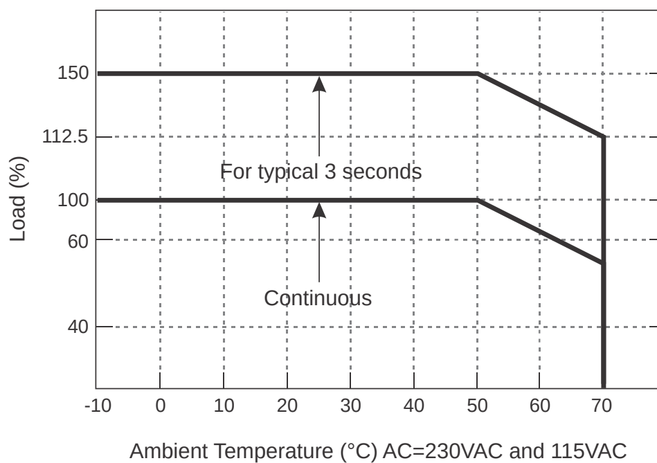
Figure 3-3 Derating Curve: Models DL150, DL240 and DL480 Series
