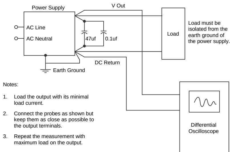
Figure 3-6 Ripple Noise Measurement Setup
