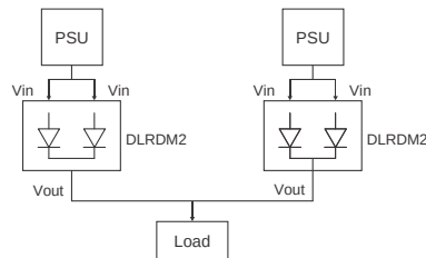
Figure 3-7 DLRDM20 Typical Applications
