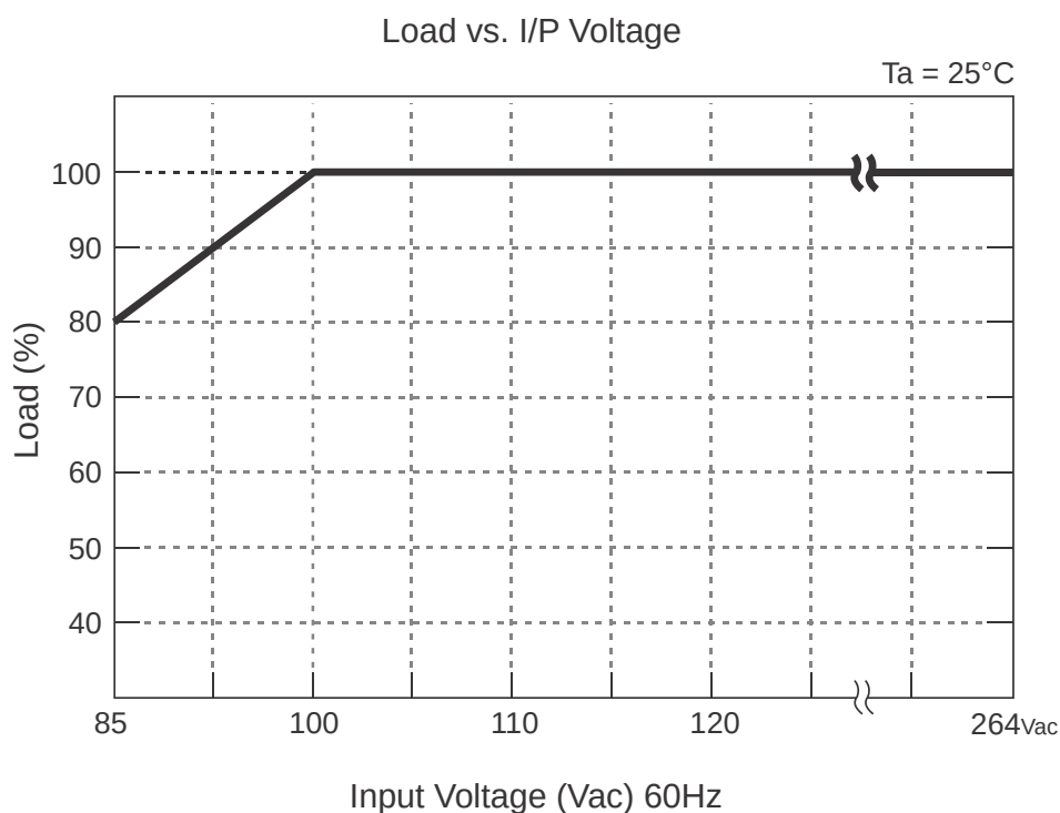
Figure 3-4 Load vs. Input Voltage: Models DL150, DL240 and DL480 Series
