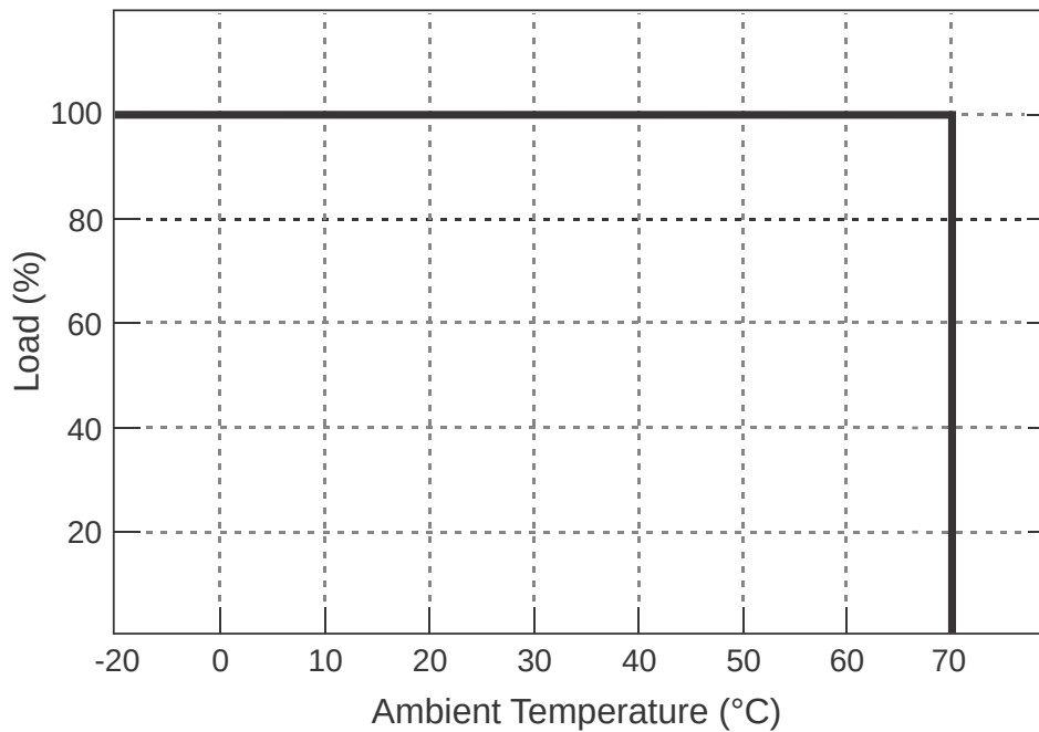
Figure 3-5 DLRDM20 Derating Curve
