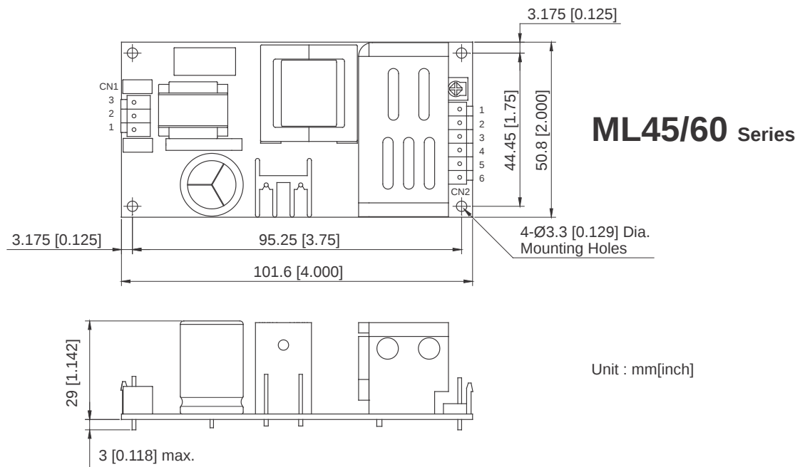
Figure 4-8 ML45/60 Dimensions
