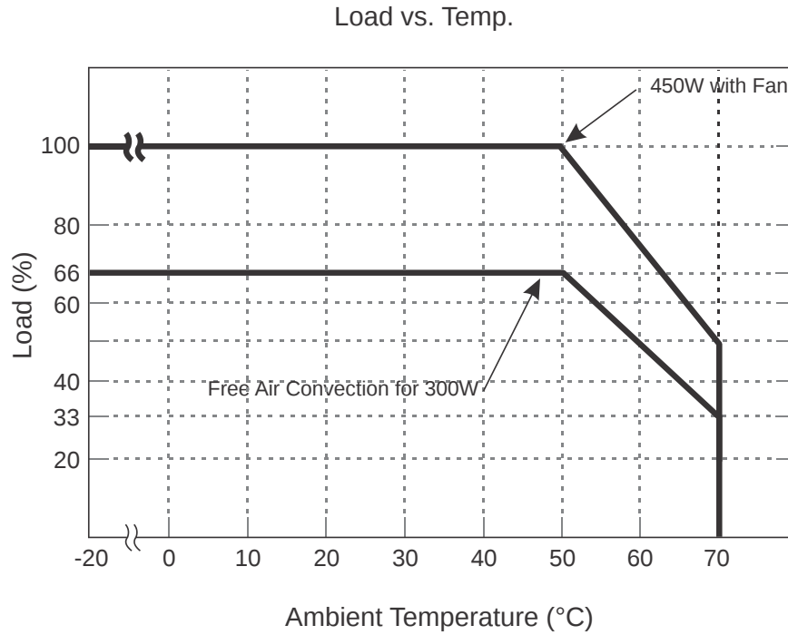
Figure 3-19 Derating Curve: Model ML450 Series
