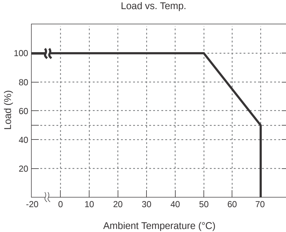
Figure 3-1 Derating Curve: Models ML05 thru ML20 Series
