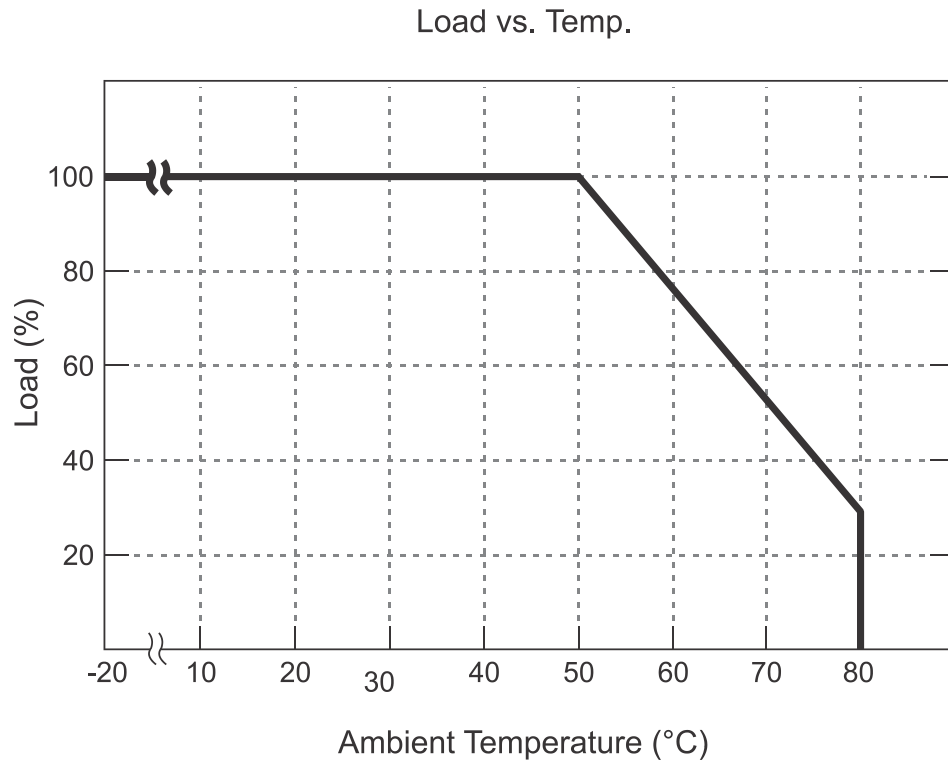
Figure 3-11 Derating Curve: Model ML100 Series
