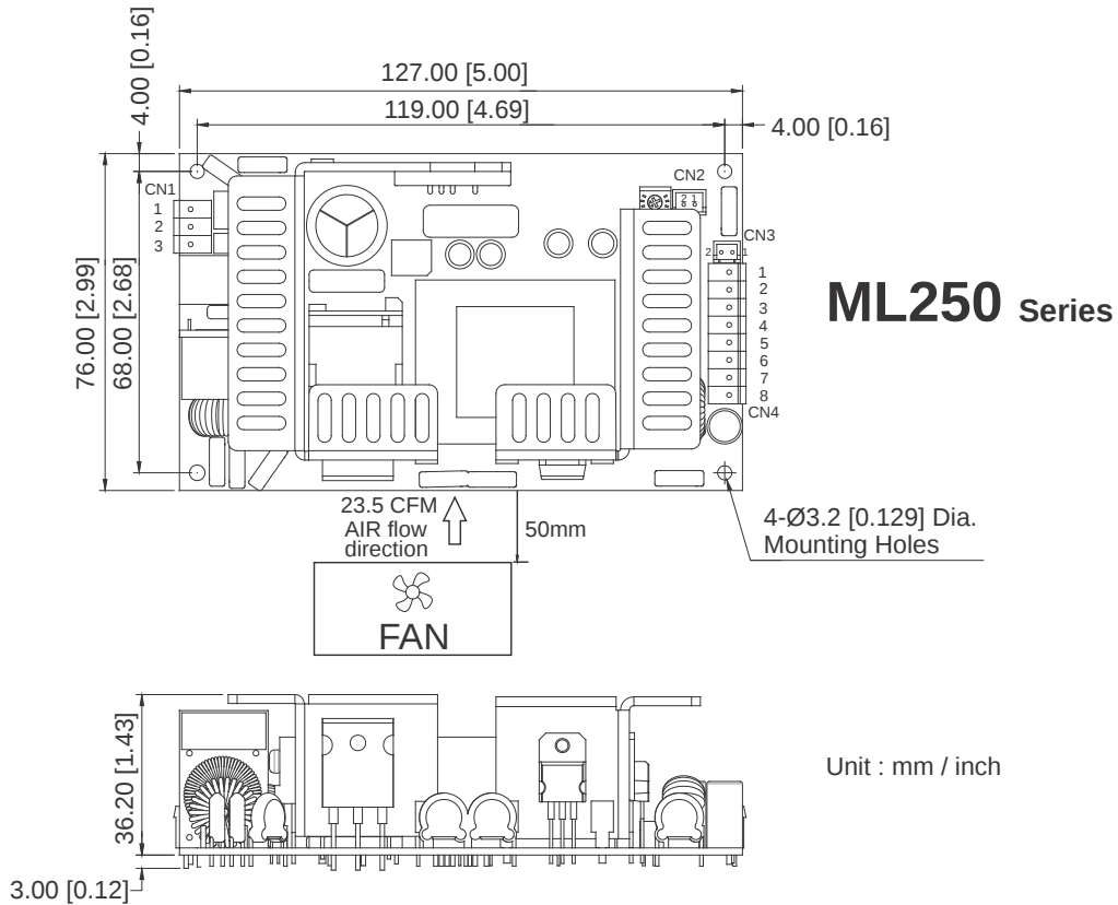
Figure 4-11 ML250 Dimensions
