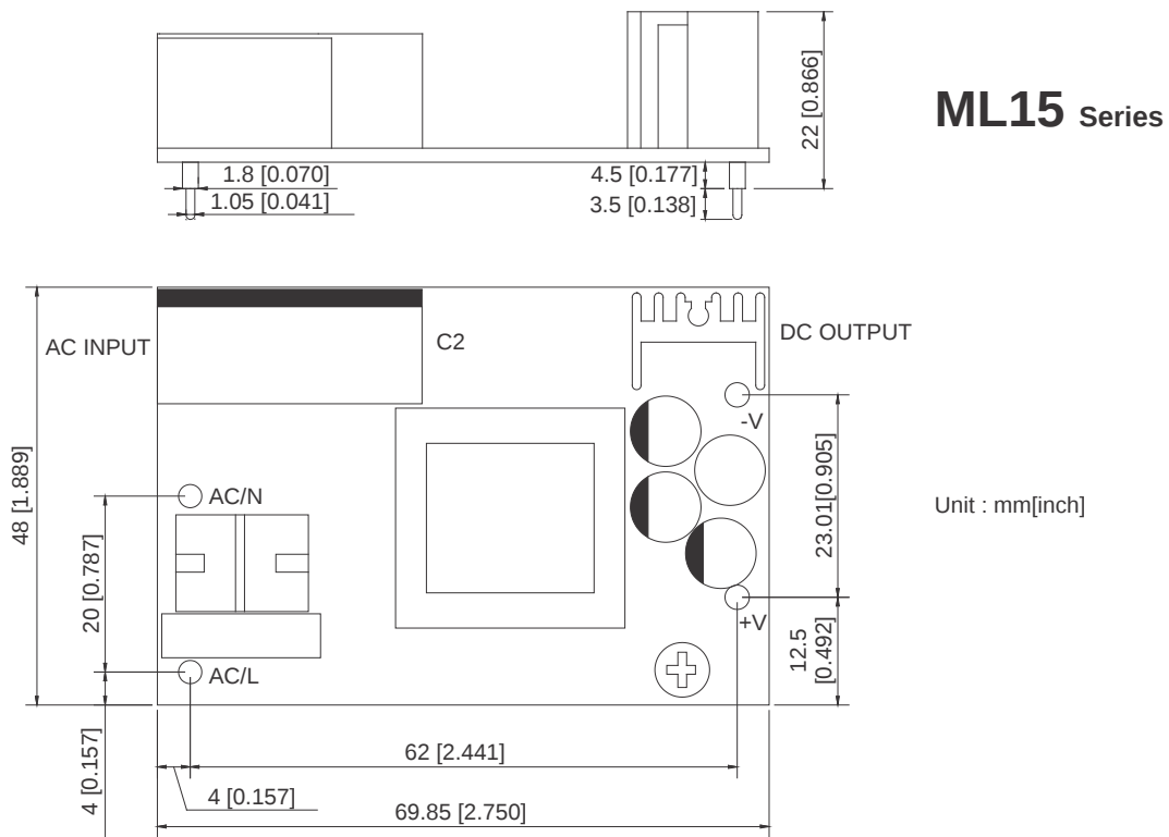
Figure 4-6 ML15 Dimensions
