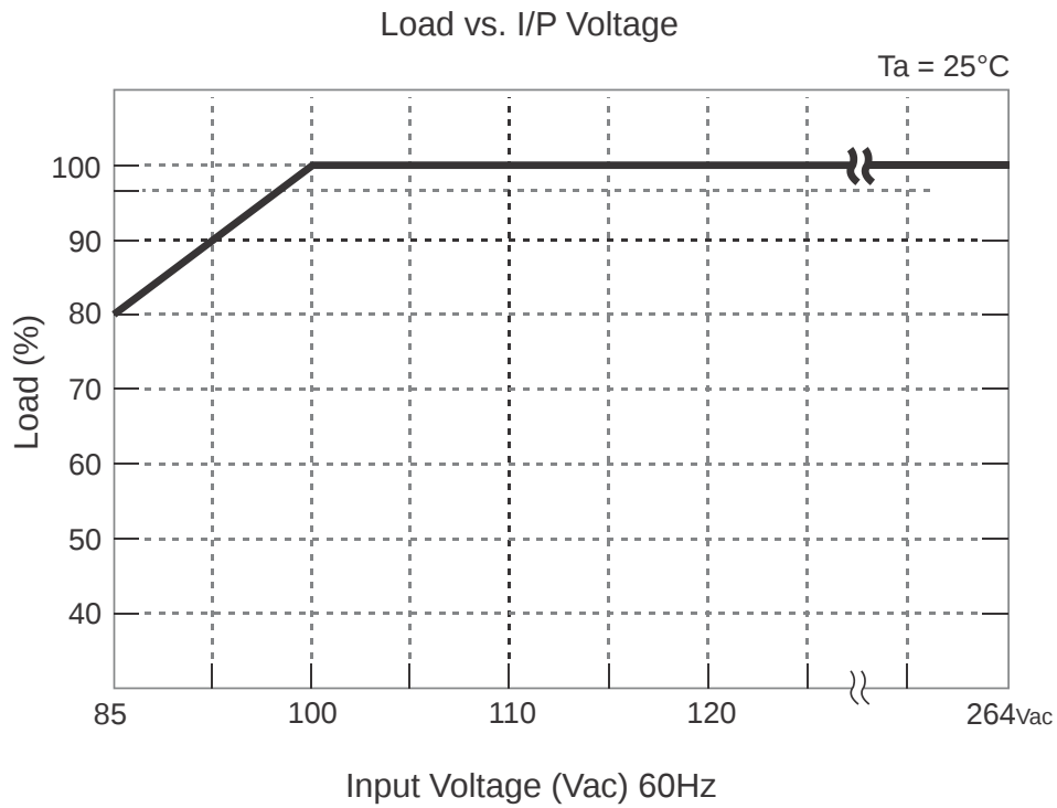
Figure 3-2 Load vs. Input Voltage: Models ML05 thru ML20 Series
