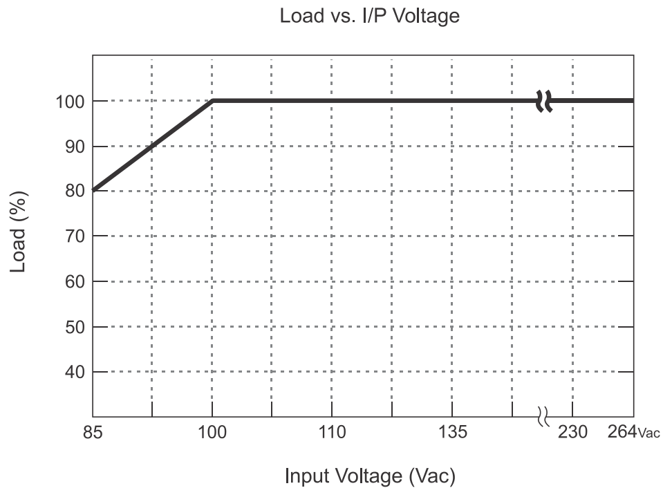
Figure 3-12 Load vs. Input Voltage: Model ML100 Series
