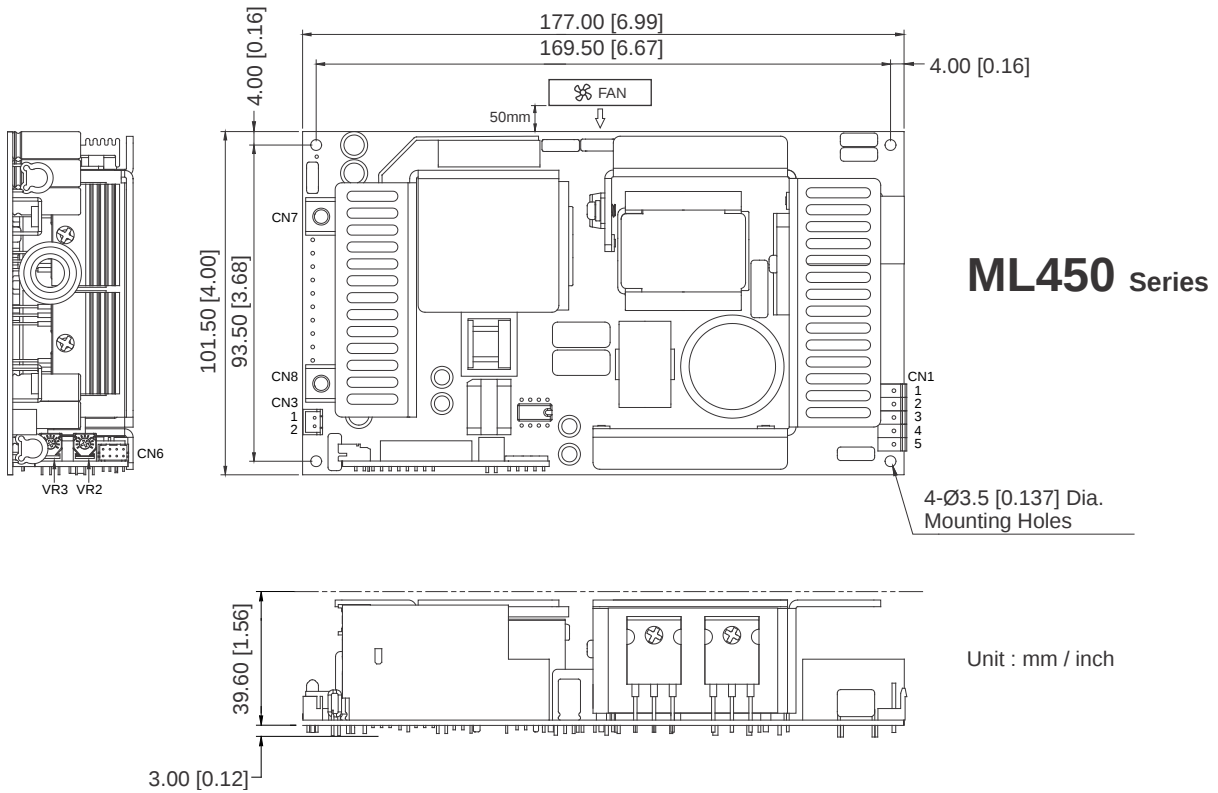
Figure 4-13 ML450 Dimensions
