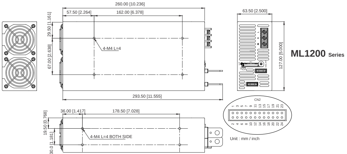
Figure 4- ML1200 Dimensions
