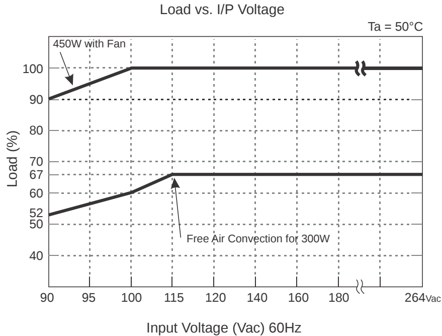
Figure 3-20 Load vs. Input Voltage: Model ML450 Series
