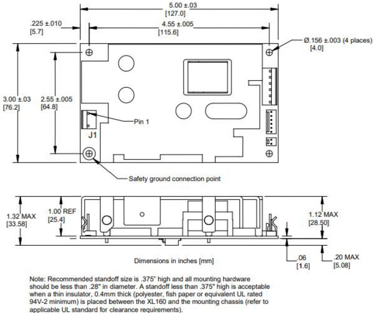
Figure 4-2 XL160 Dimensions
