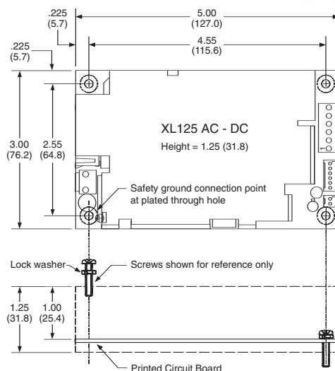
Typical Mechanical Drawing: Inches (millimeters), connectors and pinouts may vary with model. Refer to XL125 Product Specification for complete information.
