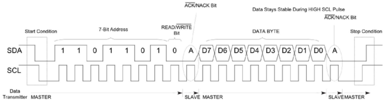
Figure 8. I²C Write Sequence Transmission
