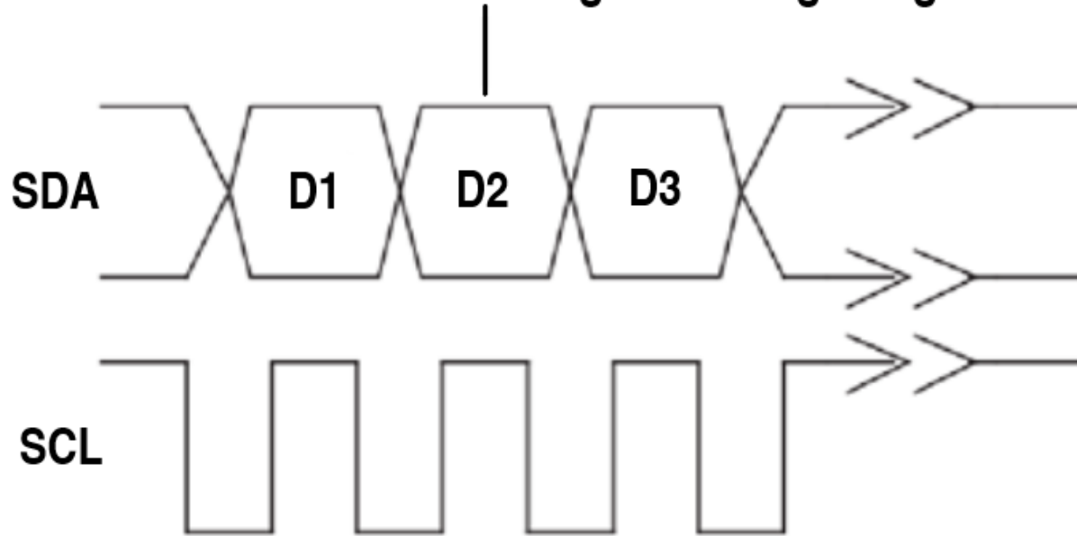
Figure 7. Bit Transition for Valid Data Bits.
