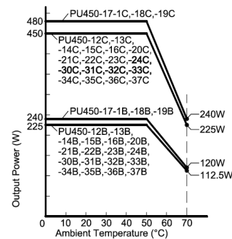
OUTPUT POWER DERATING CURVE
