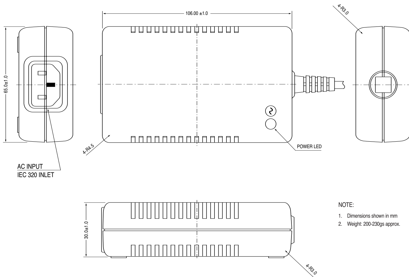
MECHANICAL DIMENSIONS mm
