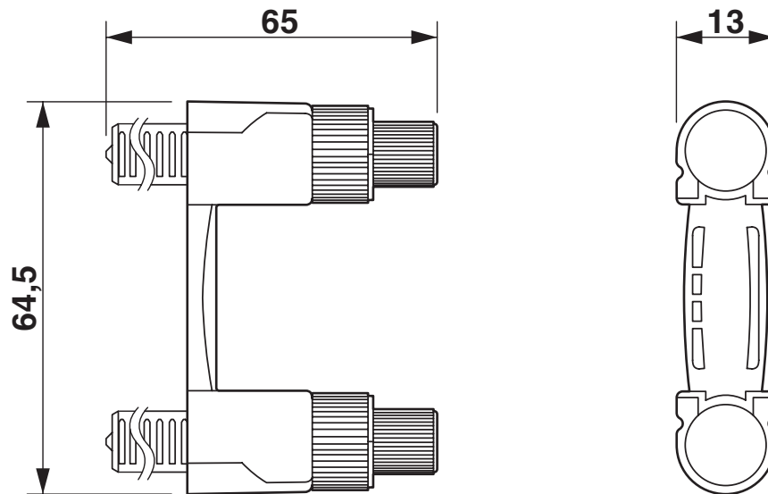
Dimensional drawing
