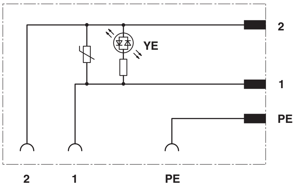
Circuit diagram
