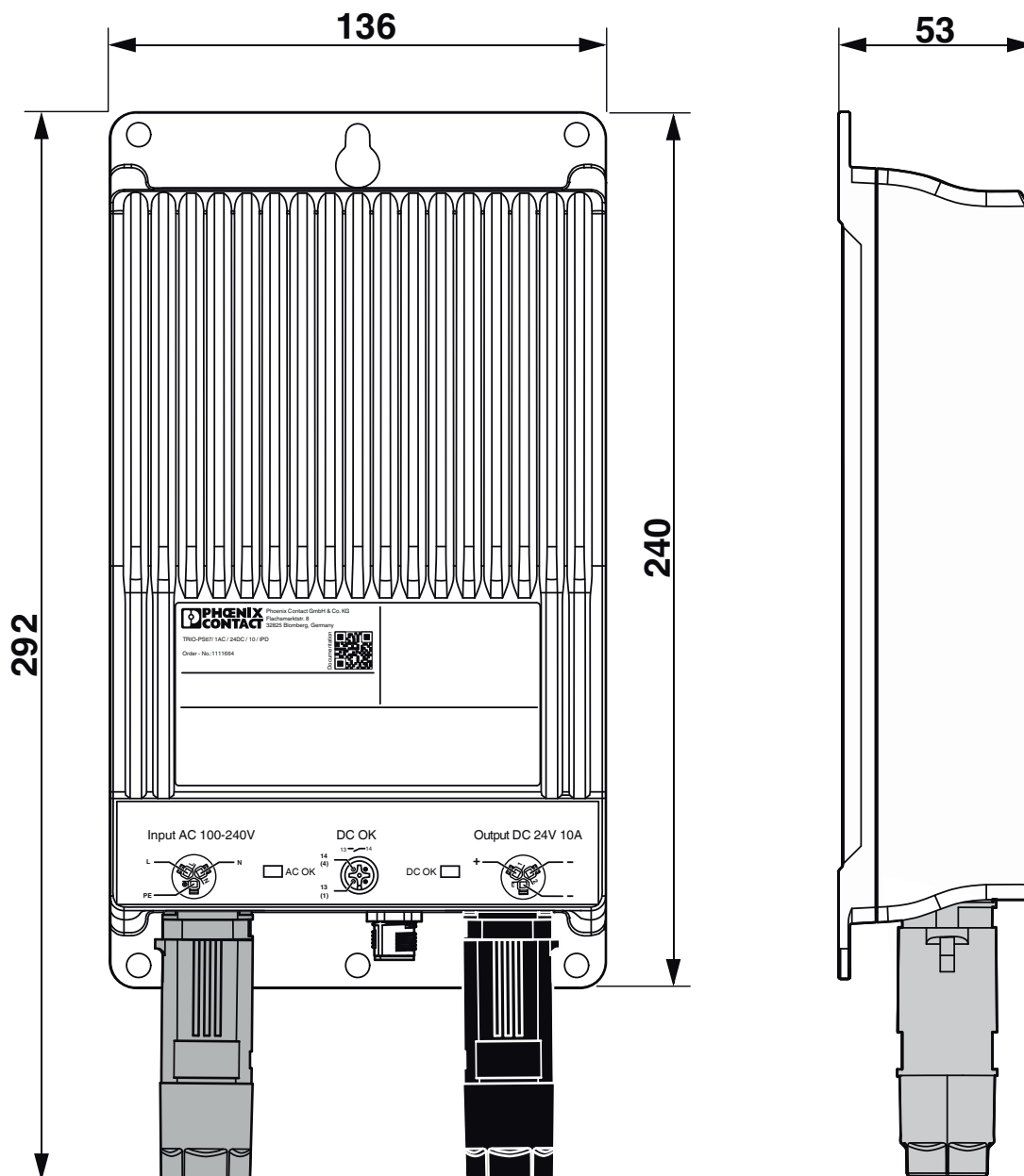
Dimensional drawing
