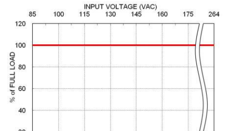
TSD40 Derating Curve vs. Input Voltage
