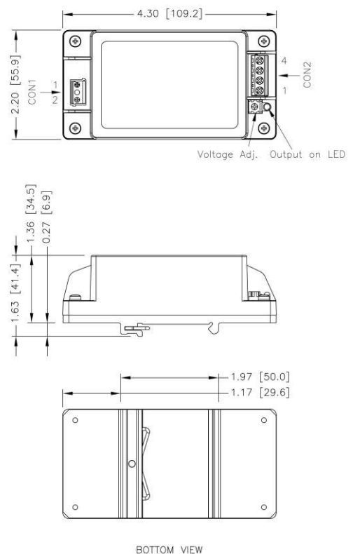
BOTTOM VIEW
