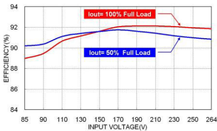
TSD40US24 Efficiency VS Input Voltage
