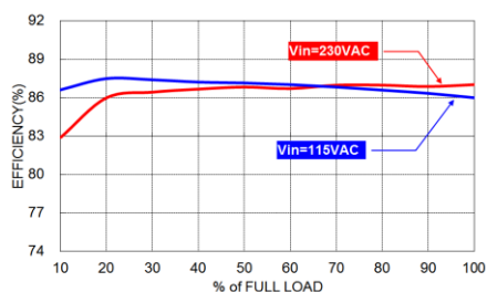
TAC15US12D Efficiency vs. Output Load
