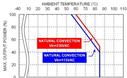
Derating Curve vs. Ambient Temperature TAC15USxxD xx=3P3/05/7P5/09/12/15/18 Connector Option : (□: JST)
