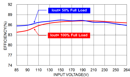
TAC15US12D Efficiency vs. Input Voltage
