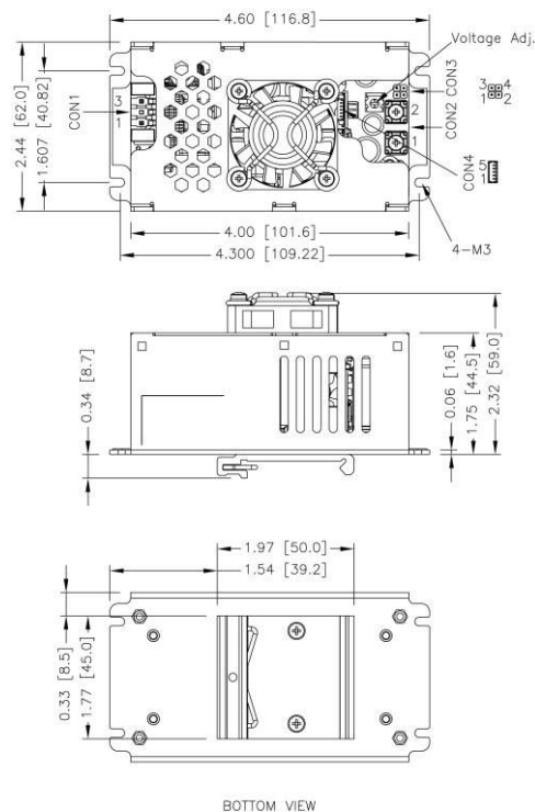
Din rail type with FAN
