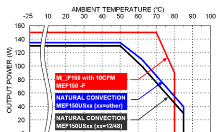
Derating Curve vs. Ambient Temperature Vin=230VAC
