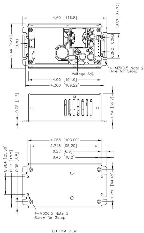
BOTTOM VIEW
