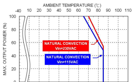
Derating Curve vs. Ambient Temperature MAC15USxxD xx=24/28/36/48/53 Connector Option : (Blank: JST)
