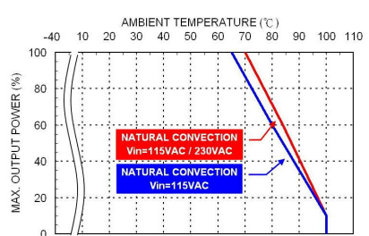
Derating Curve vs. Ambient Temperature MAC15USxxD xx=24/28/36/48/53 Connector Option : (-M / -T / -D)
