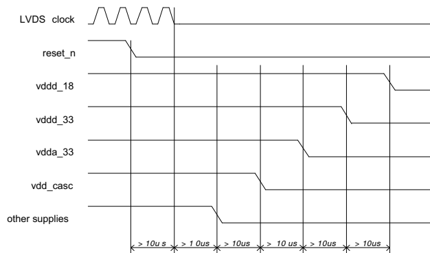
Figure 15. Power-down Sequence
