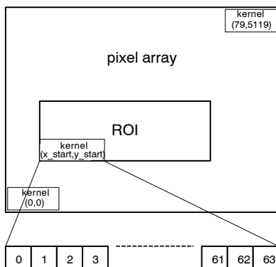
Figure 35. Kernel Organization in Pixel Array
