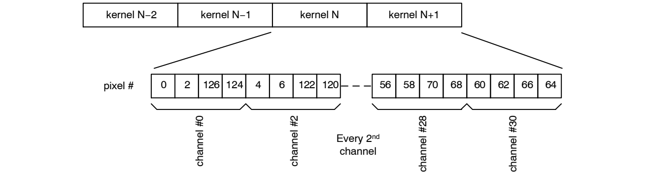
Figure 41. Data Output Order for 16 LVDS Output Channels in Subsampling Mode on a Monochrome Sensor
