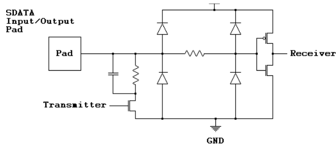
Figure 46. Serial Interface
