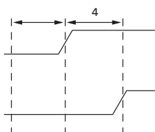
Figure 23: Serial Host Interface Stop Condition Timing
