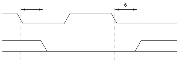
Figure 27: Acknowledge Signal Timing After an 8-Bit Read from the Sensor
