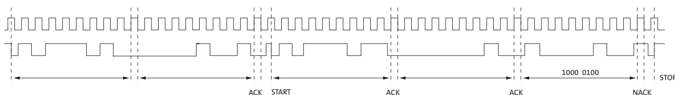
Figure 20: Timing Diagram Showing a Read from Reg0x09; Returned Value 0x0284
