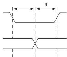
Figure 24: Serial Host Interface Data Timing for Write
