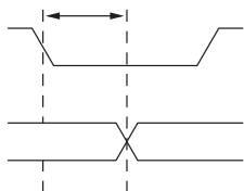
Figure 25: Serial Host Interface Data Timing for Read
