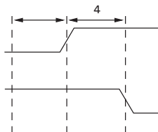
Figure 22: Serial Host Interface Start Condition Timing
