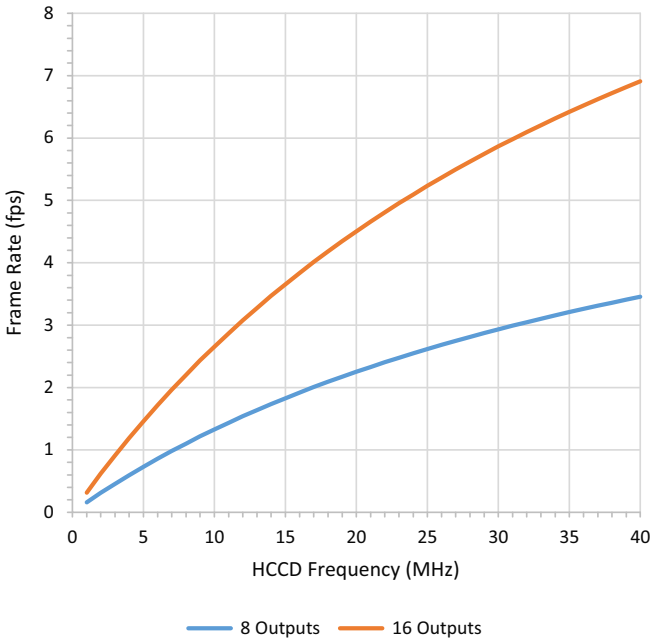
Figure 14. Frame Rates
