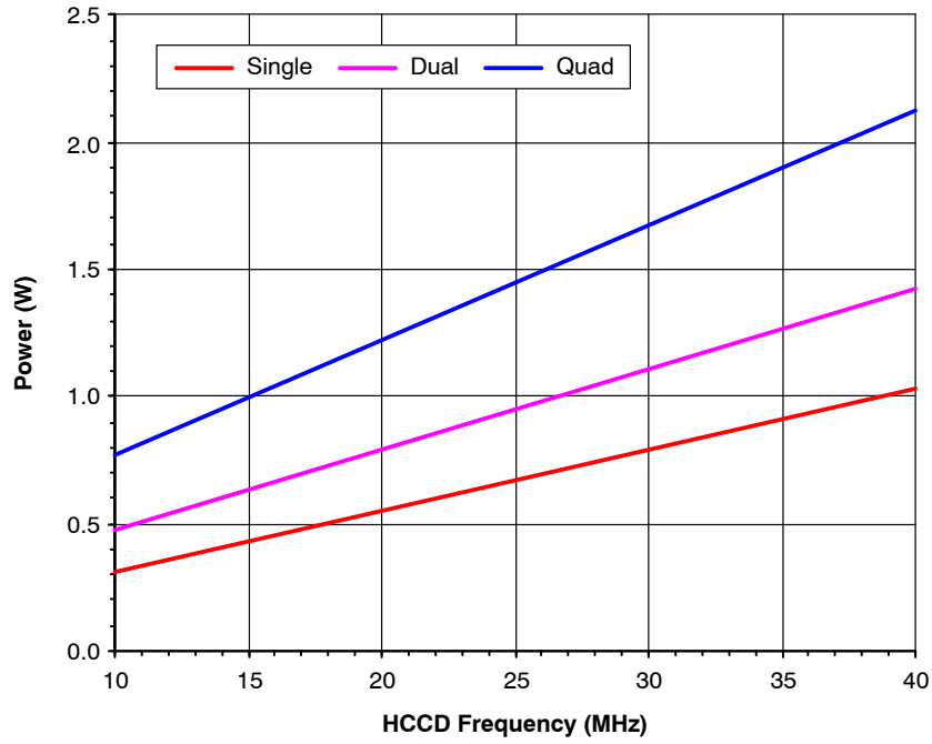
Figure 11. Power
