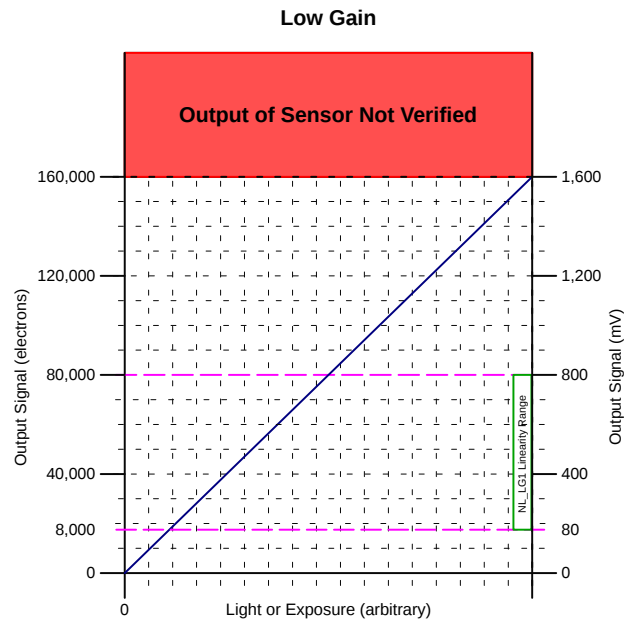
Figure 7. Low Gain Linear Signal Range
