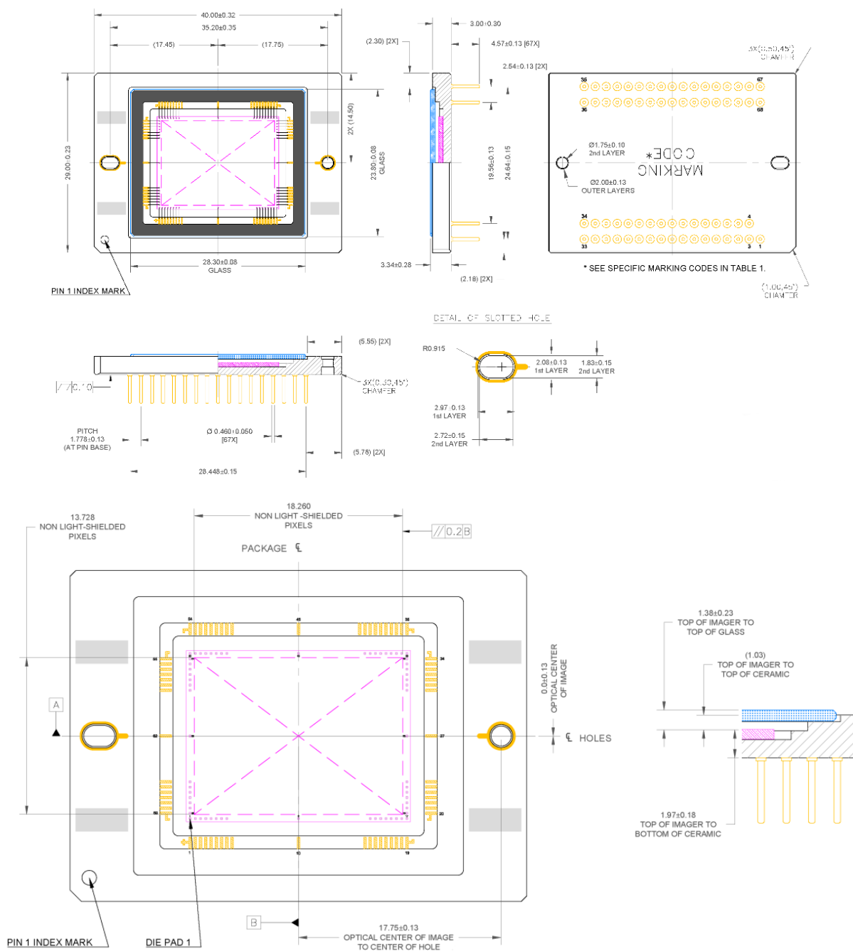
Figure 24. Completed Assembly
