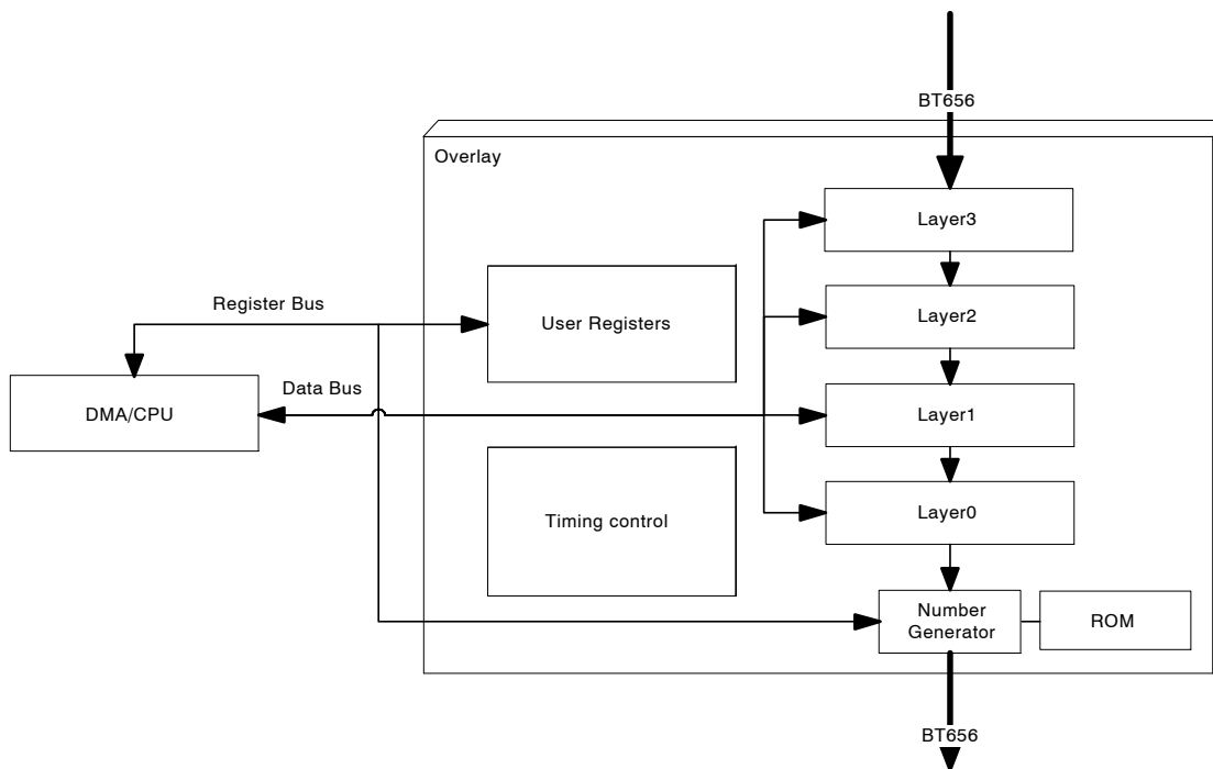
Figure 26. Internal Block Diagram Overlay
