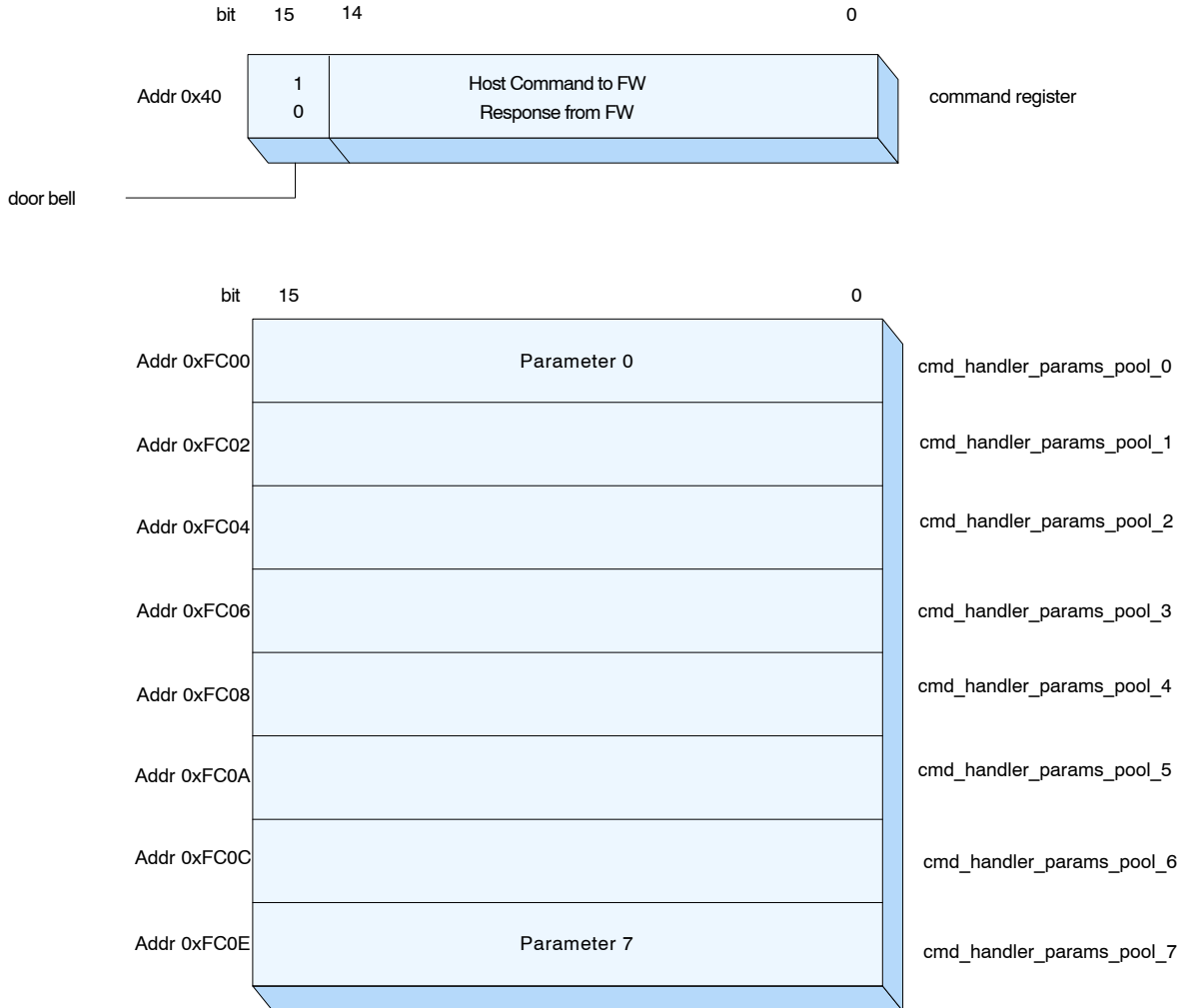
Figure 15. Interface Structure
