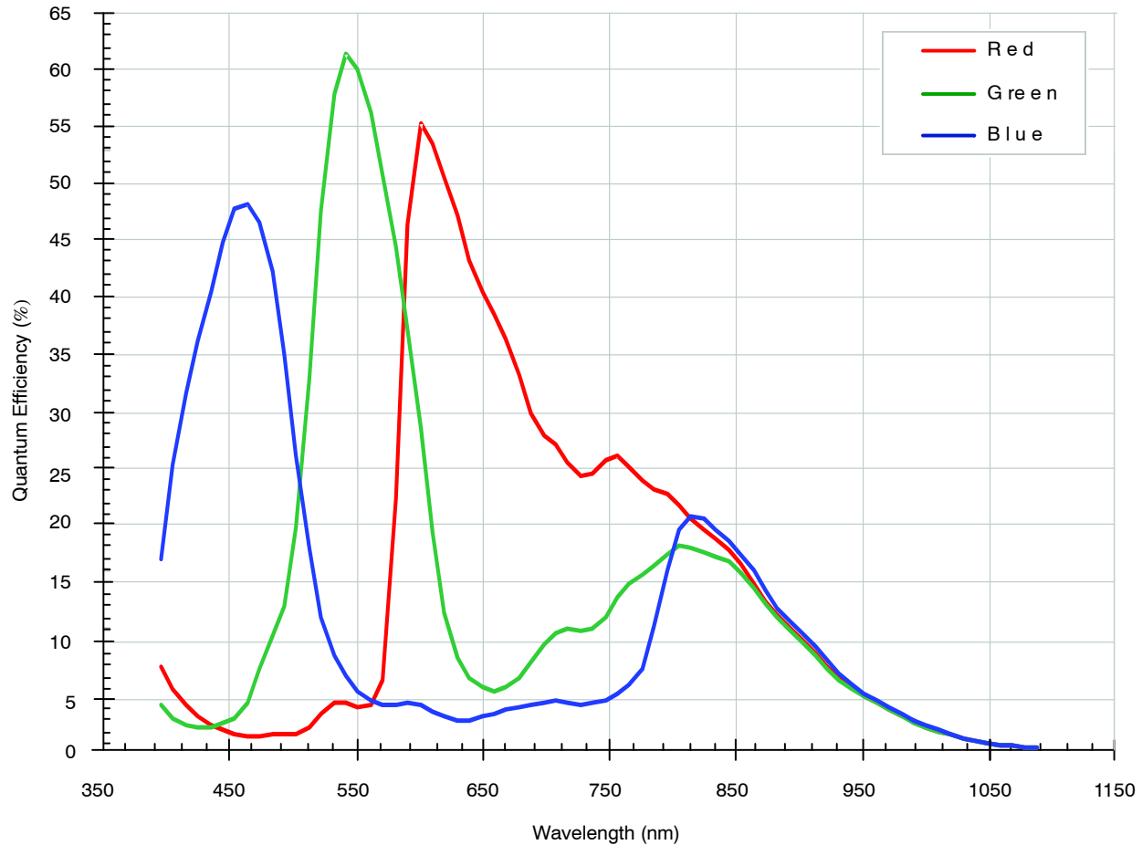
Figure 43. Quantum Efficiency
