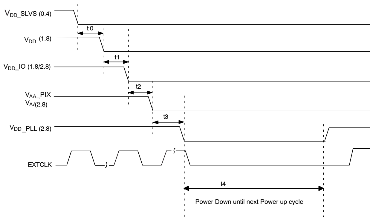
Figure 47. Power Down
