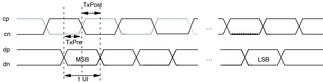
Figure 11. Timing Diagram
