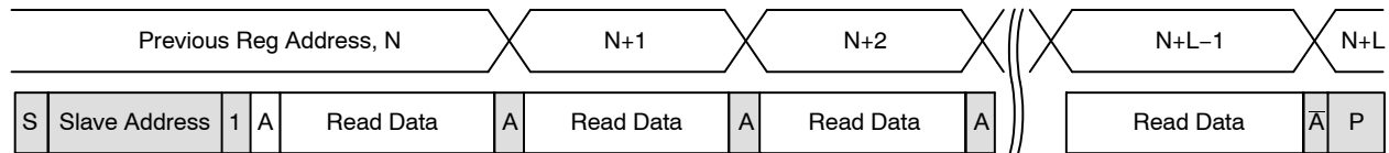
Figure 40. Sequential READ, Start from Current Location
