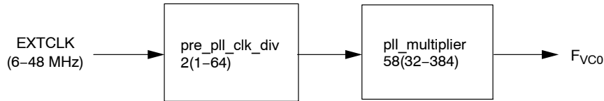
Figure 20. PLL Dividers Affecting VCO Frequency
