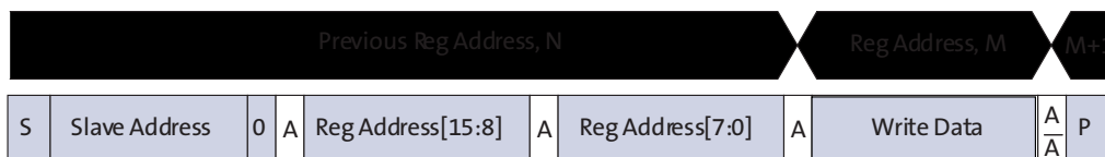
Figure 46: Single WRITE to Random Location
