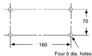
Mounting holes Side mounting
