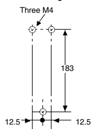
Mounting holes
