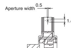
Cross section view A-A (Detector side)
