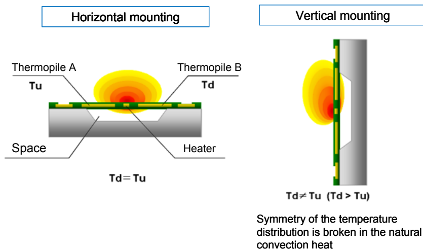
Fig.20 Influence of mounting direction of the sensor chip
