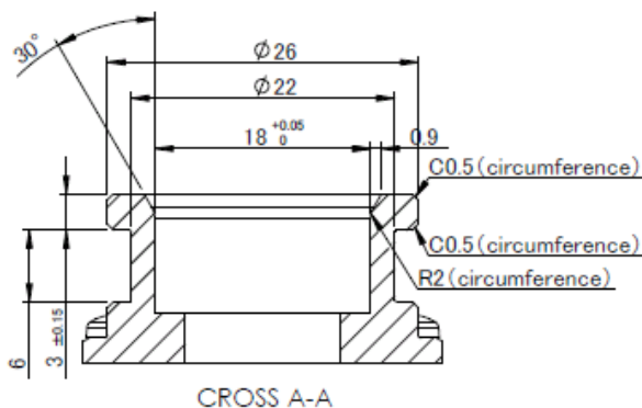
Fig.10 Quick fastener P14 Outline Dimensions
