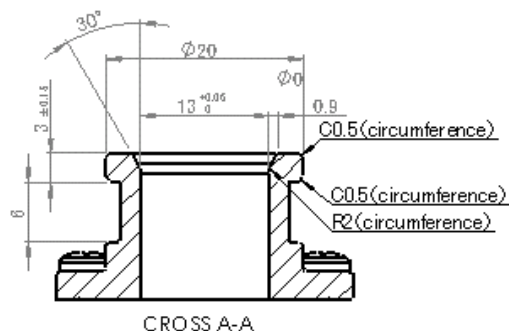
Fig.9 Quick fastener P10 Outline Dimensions
