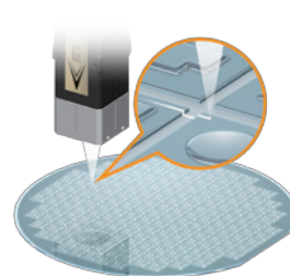
Gap measurement of electronic chips
