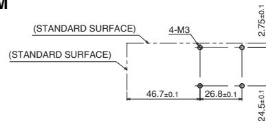
MOUNTING SCREW HOLES
