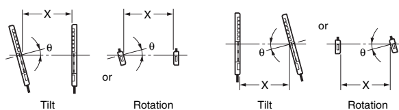
(1) Emitter Angle Characteristics (2) Receiver Angle Characteristics
