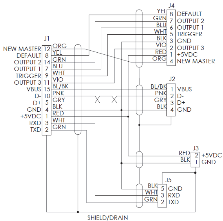
SCHEMATIC
