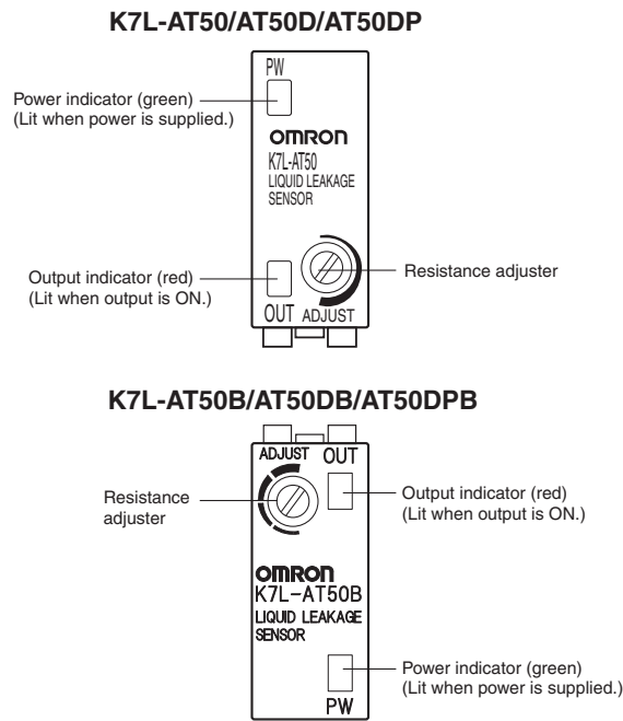
Setting Sensing Range
