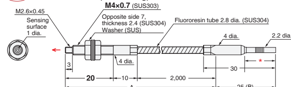
(45-D) E32-T61-S 2M (No Cutting)
