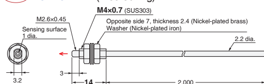
(45-A) E32-T51R 2M (Free Cutting)
