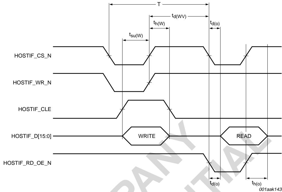
Fig 18. Host interface timing
