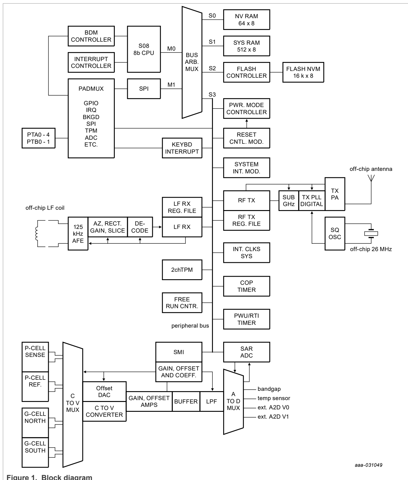
Figure 1. Block diagram
