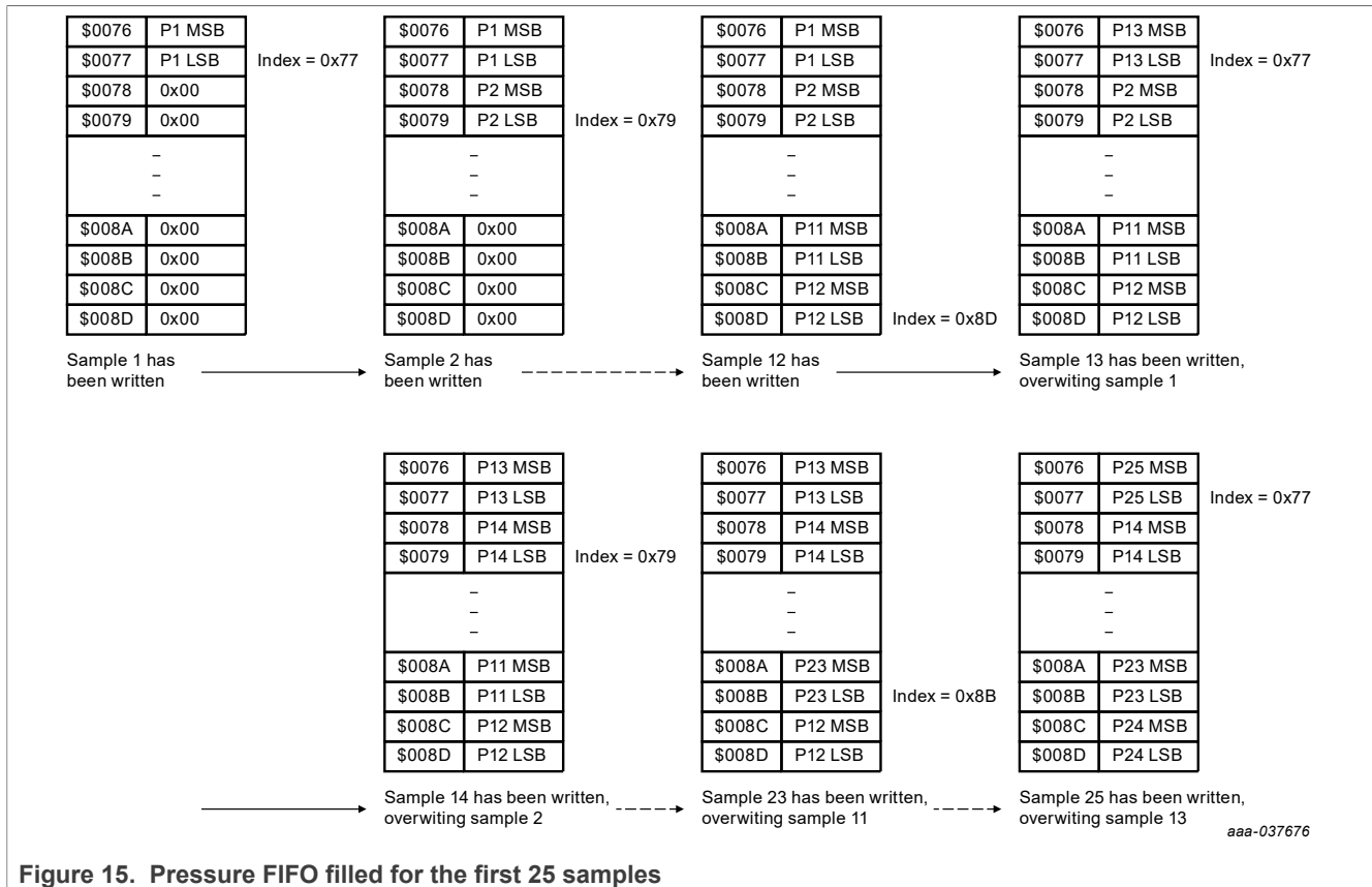
Figure 15. Pressure FIFO filled for the first 25 samples
