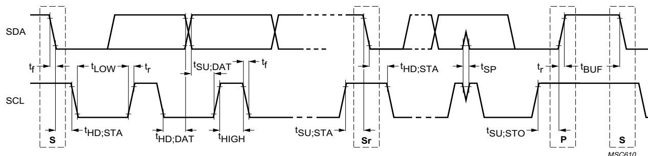
Fig 5. I 2 C slave timing diagram
