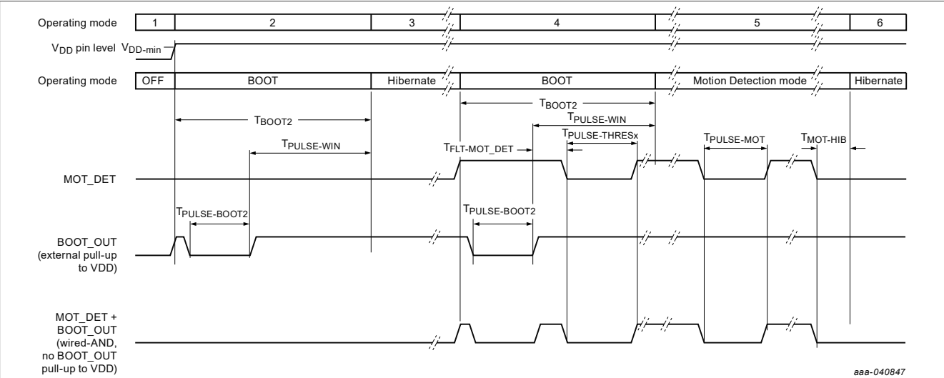
Figure 18. BOOT2 sequence and One-wire motion-detection protocol diagram (BT_MODE = V DD )
