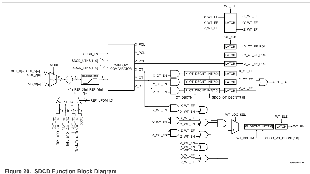
Figure 20. SDCD Function Block Diagram
