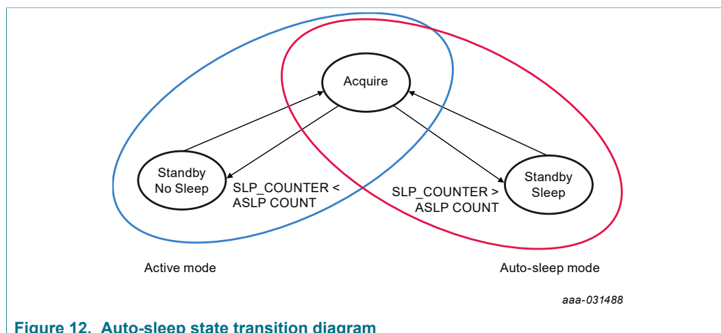
Figure 12. Auto-sleep state transition diagram
